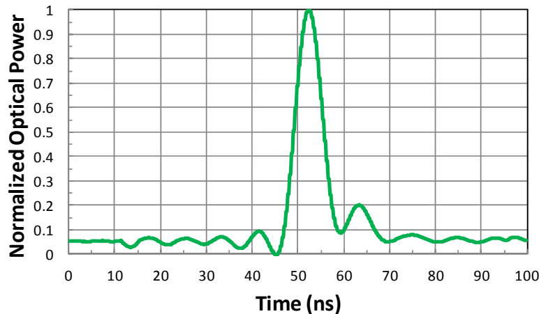
Figure 6 Temporal response of a high power VCSEL showing rise and fall times less than 1ns
